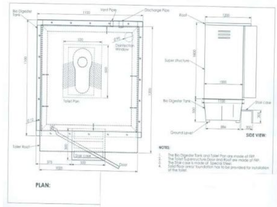
Figure 8: Details of Bio-Toilet (Source: Private Agency)
